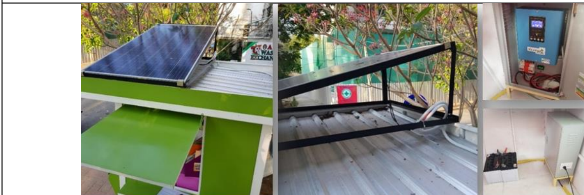
Solar PV Power for Electricity in a Waste Bank (ARU, Thailand)
